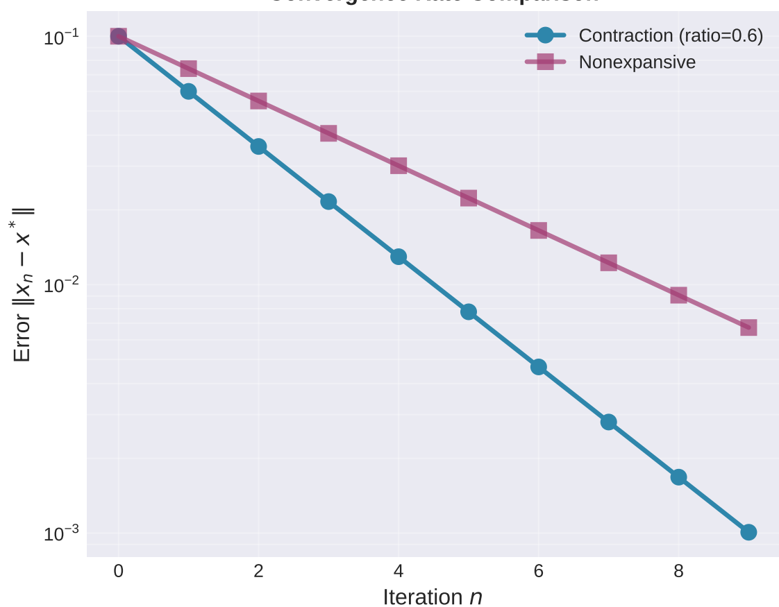
Convergence Rate Comparison
