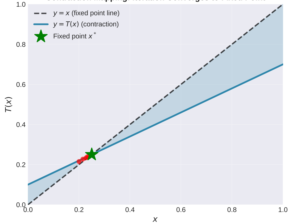
Contraction Mapping: Iteration Converges to Fixed Point
