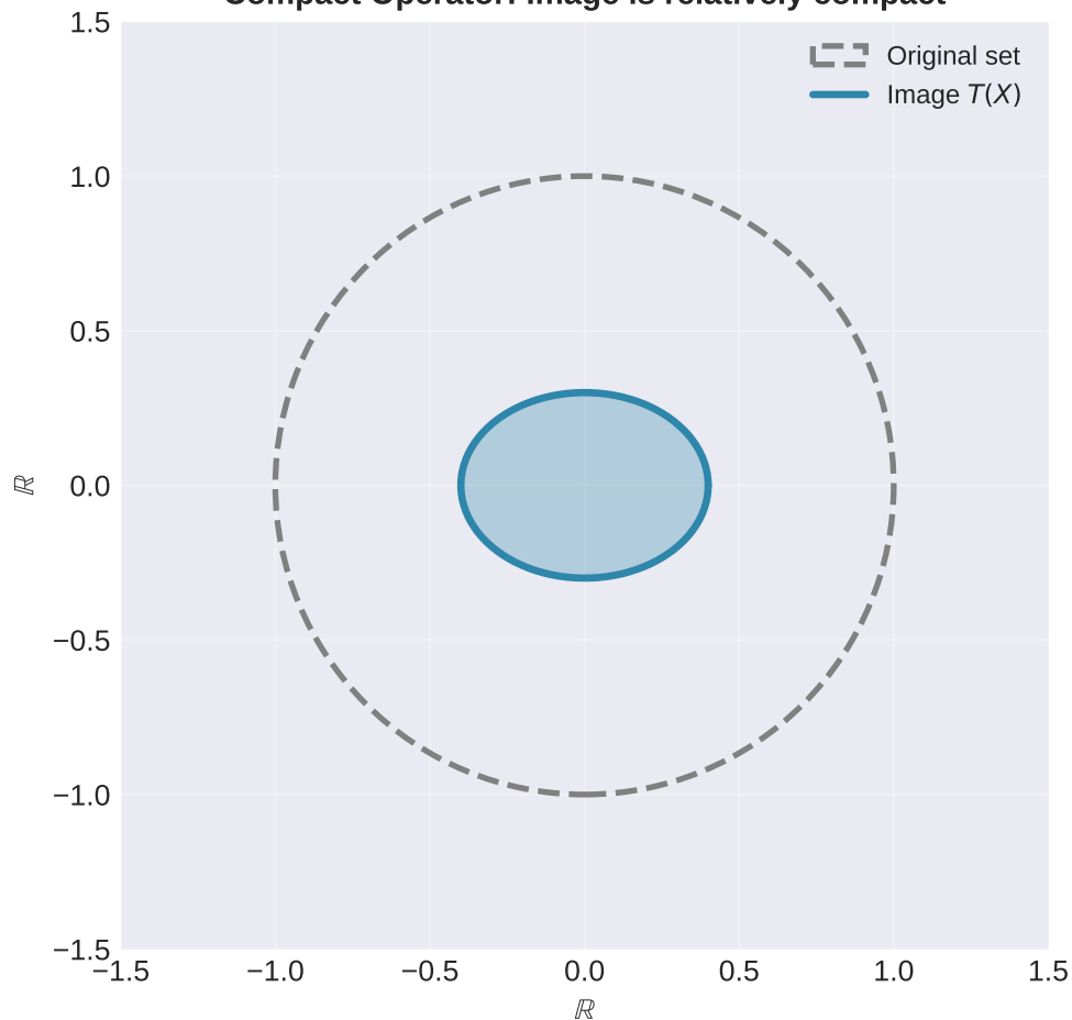
Compact Operator: Image is relatively compact
