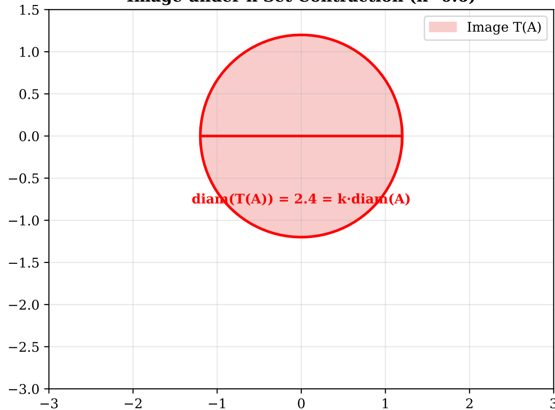
Image under k-Set Contraction (k=0.6)
