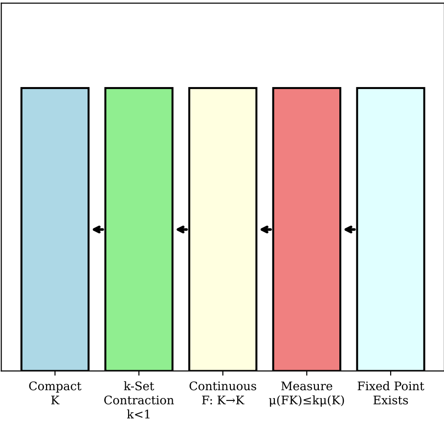
Darbo's Fixed Point Theorem: Chain of Implications
