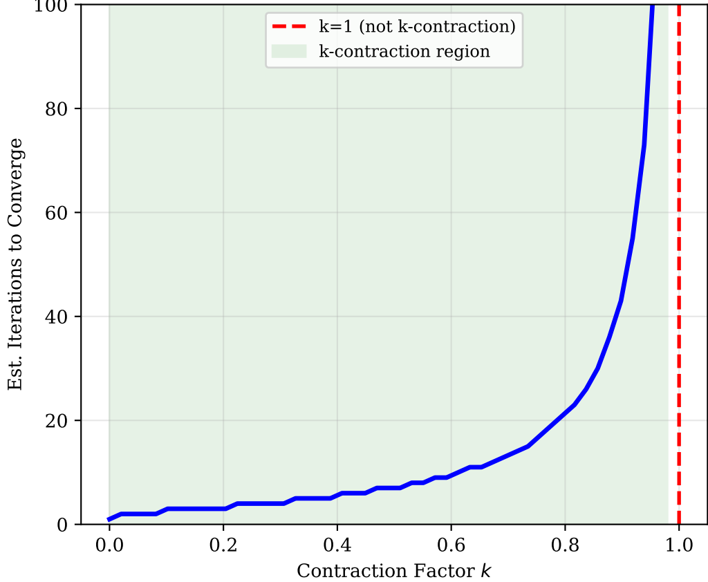
Property 3: Contraction Principle ( k < 1 )
