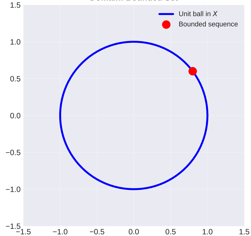
Domain: Bounded Set
