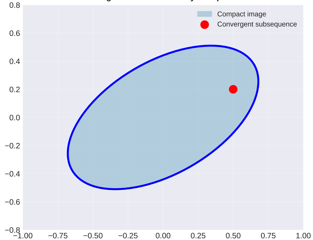
Image under T : Relatively Compact
