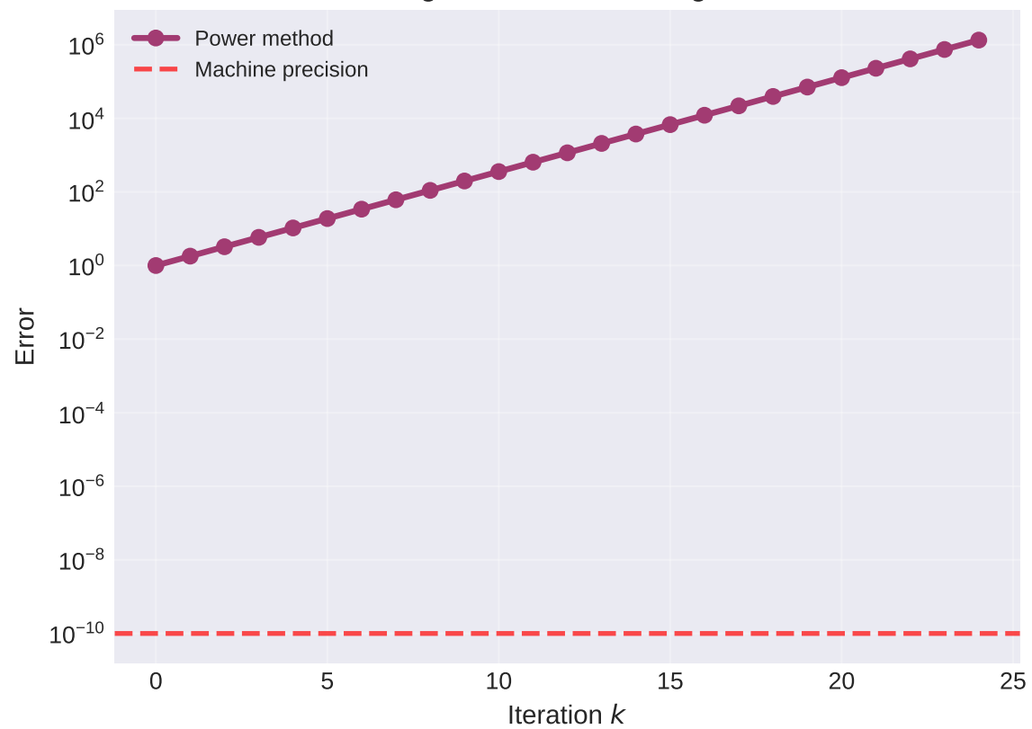
Convergence to Dominant Eigenvalue
