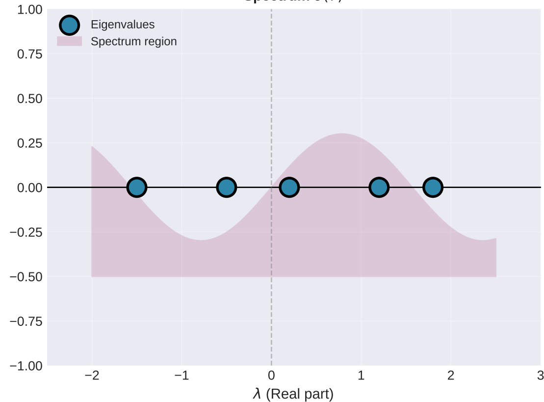
Spectrum \sigma(T)
