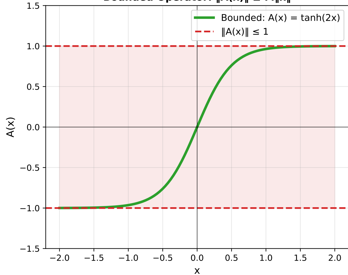
Bounded Operator: \|A(x)\| \leq M\|x\|
