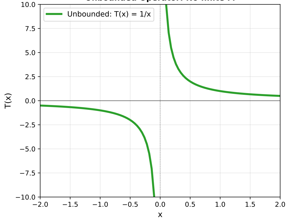
Unbounded Operator: No finite M
