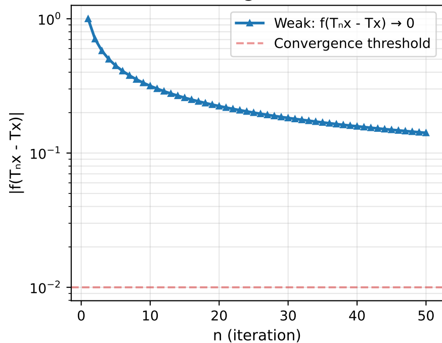
Weak Convergence (Slowest)
