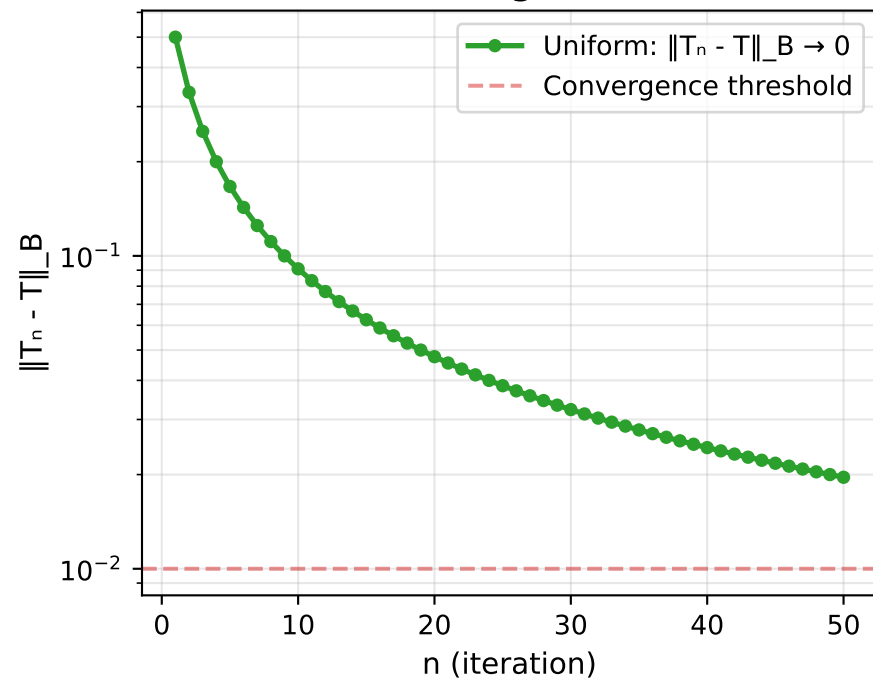
Uniform Convergence (Fastest)
