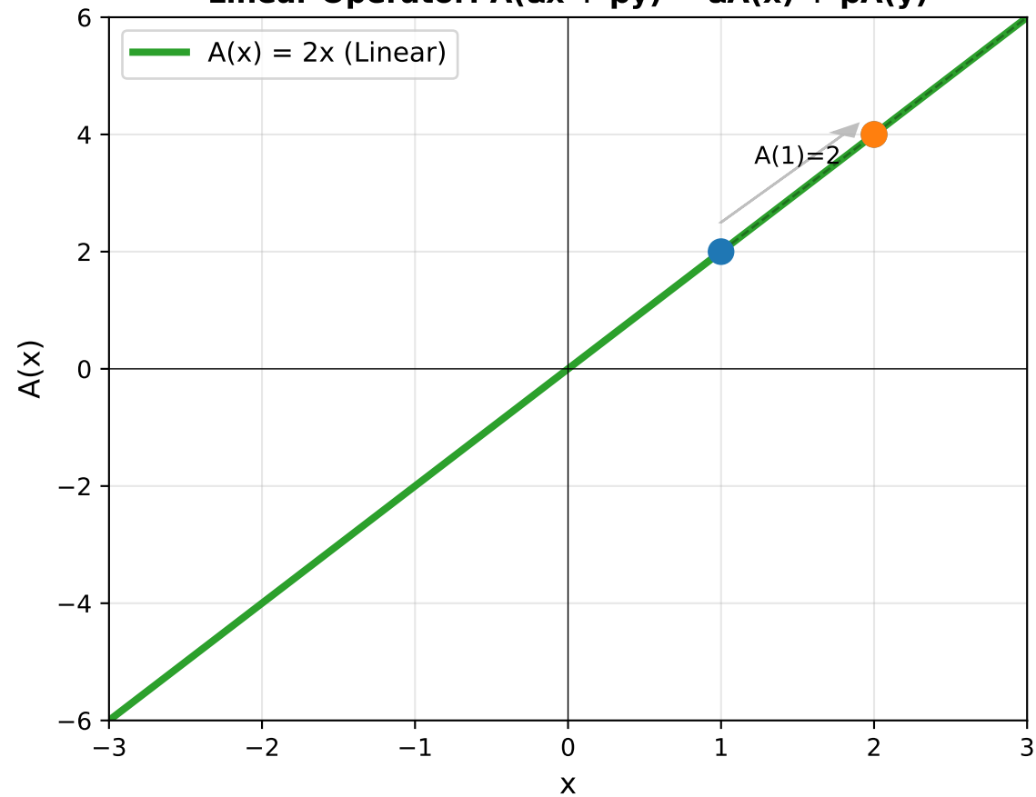
Linear Operator: A(\alpha x + \beta y) = \alpha A(x) + \beta A(y)
