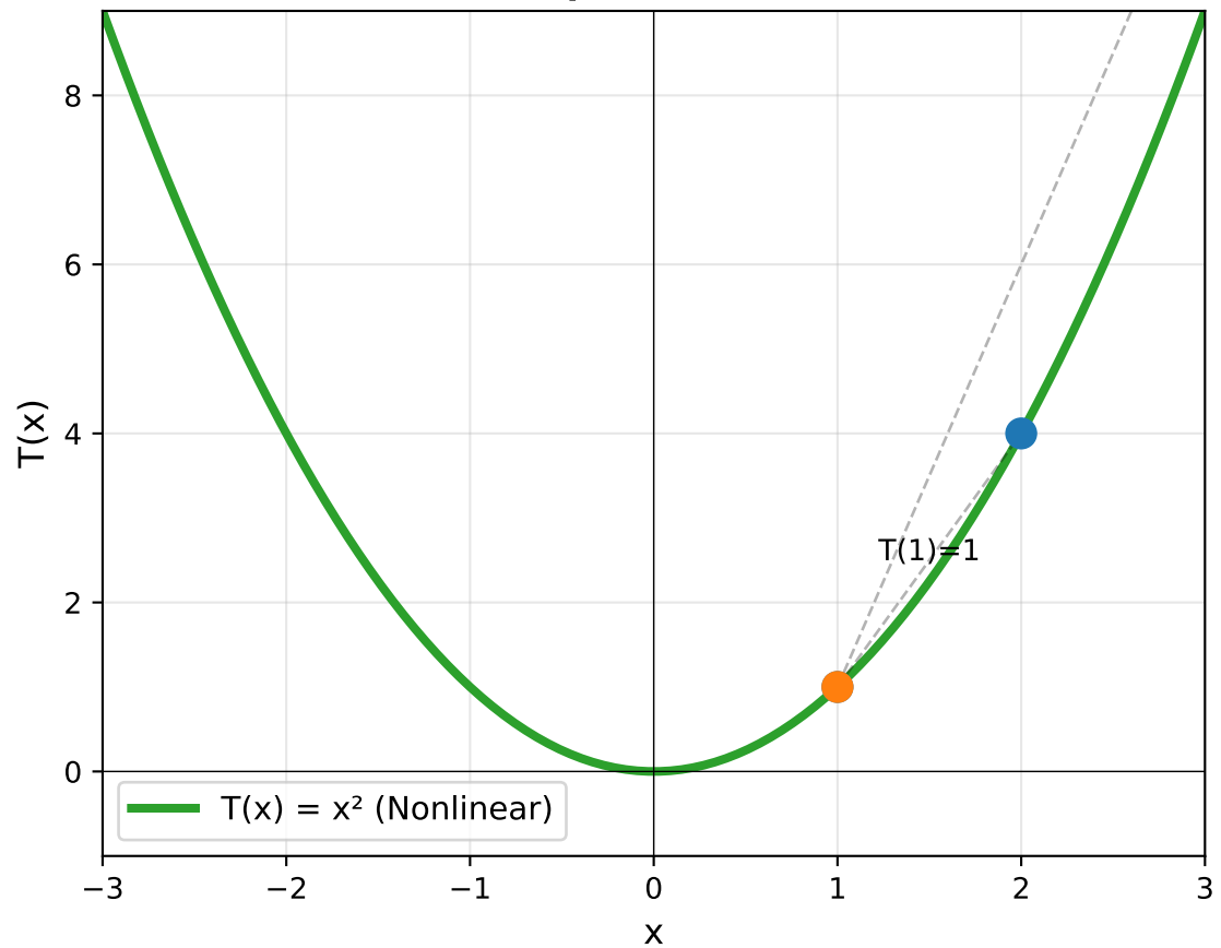
Nonlinear Operator: T(x) \neq \alpha T(x)
