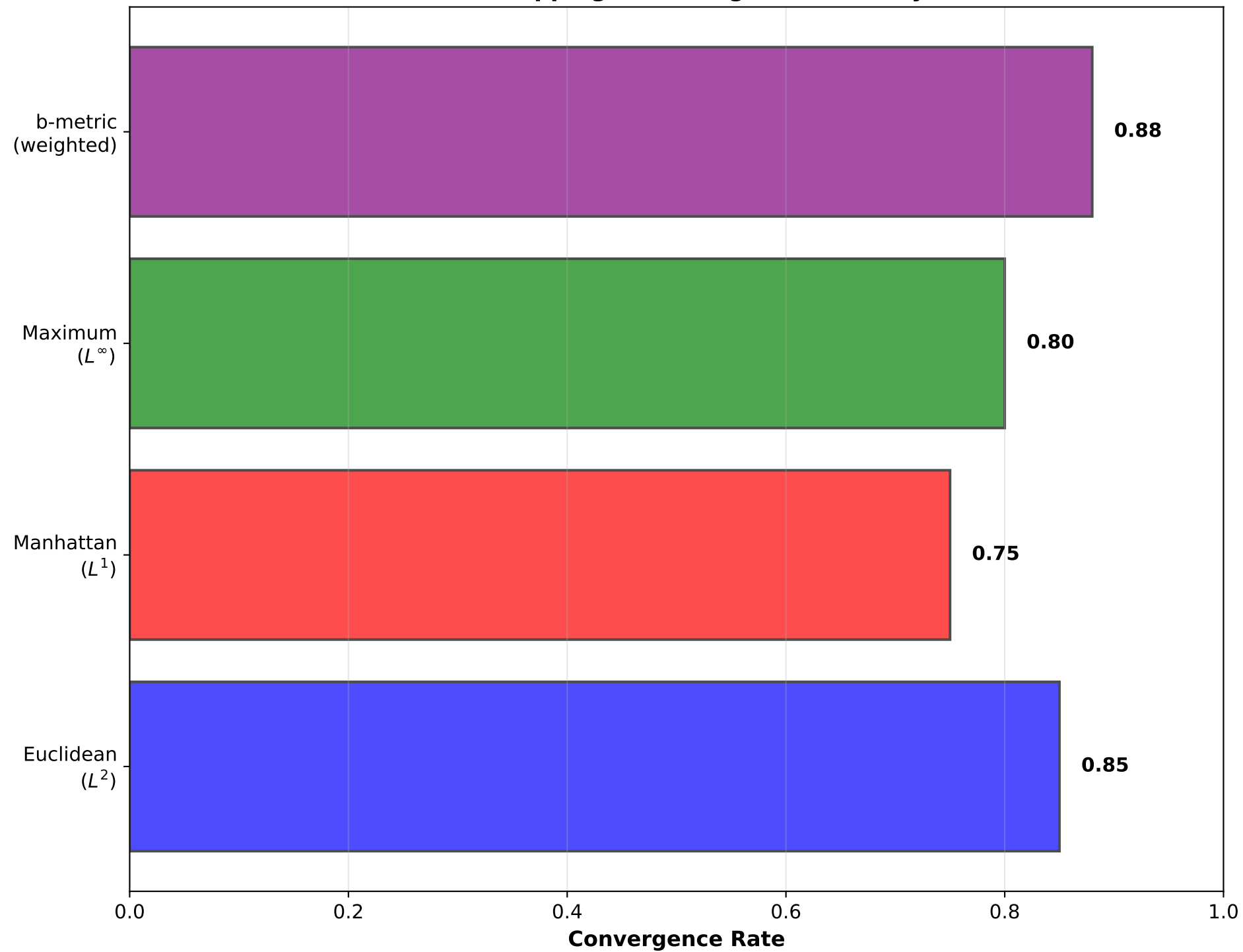
Contraction Mappings: Convergence Rates by Metric
