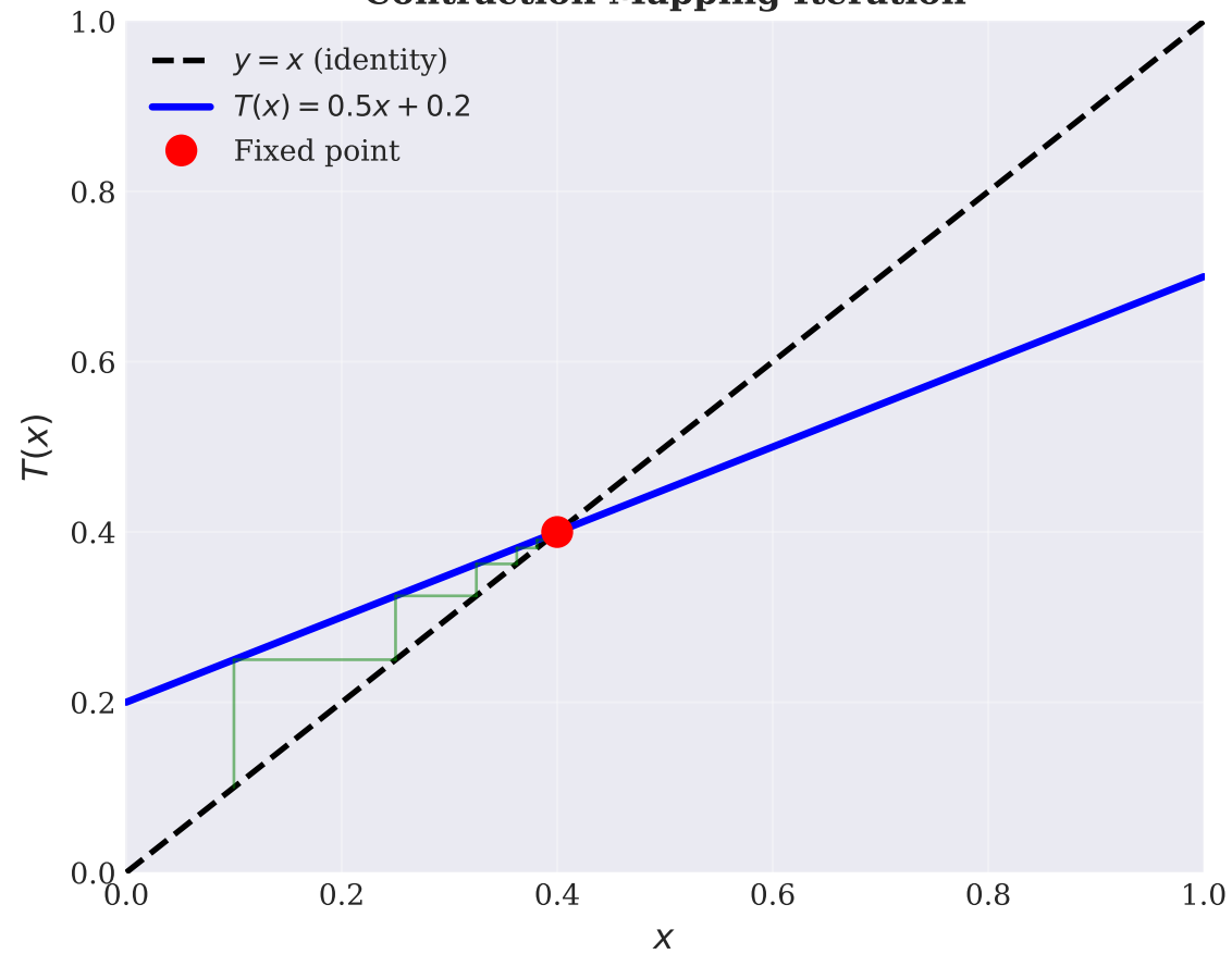
Contraction Mapping Iteration
