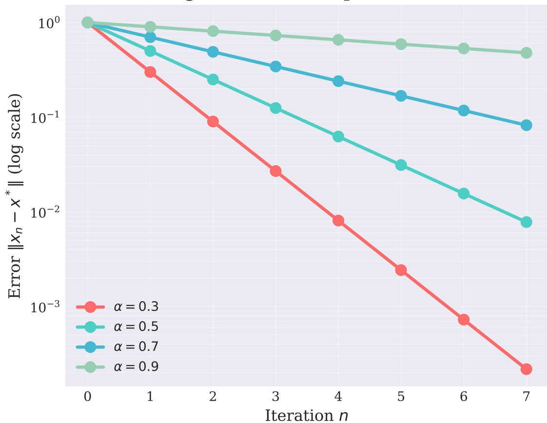
Convergence: Effect of Lipschitz Constant
