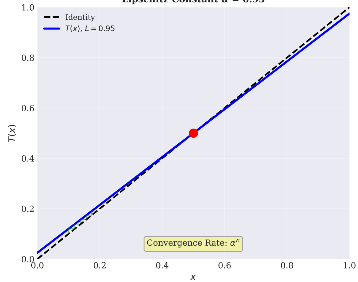
Lipschitz Constant \alpha = 0.95
