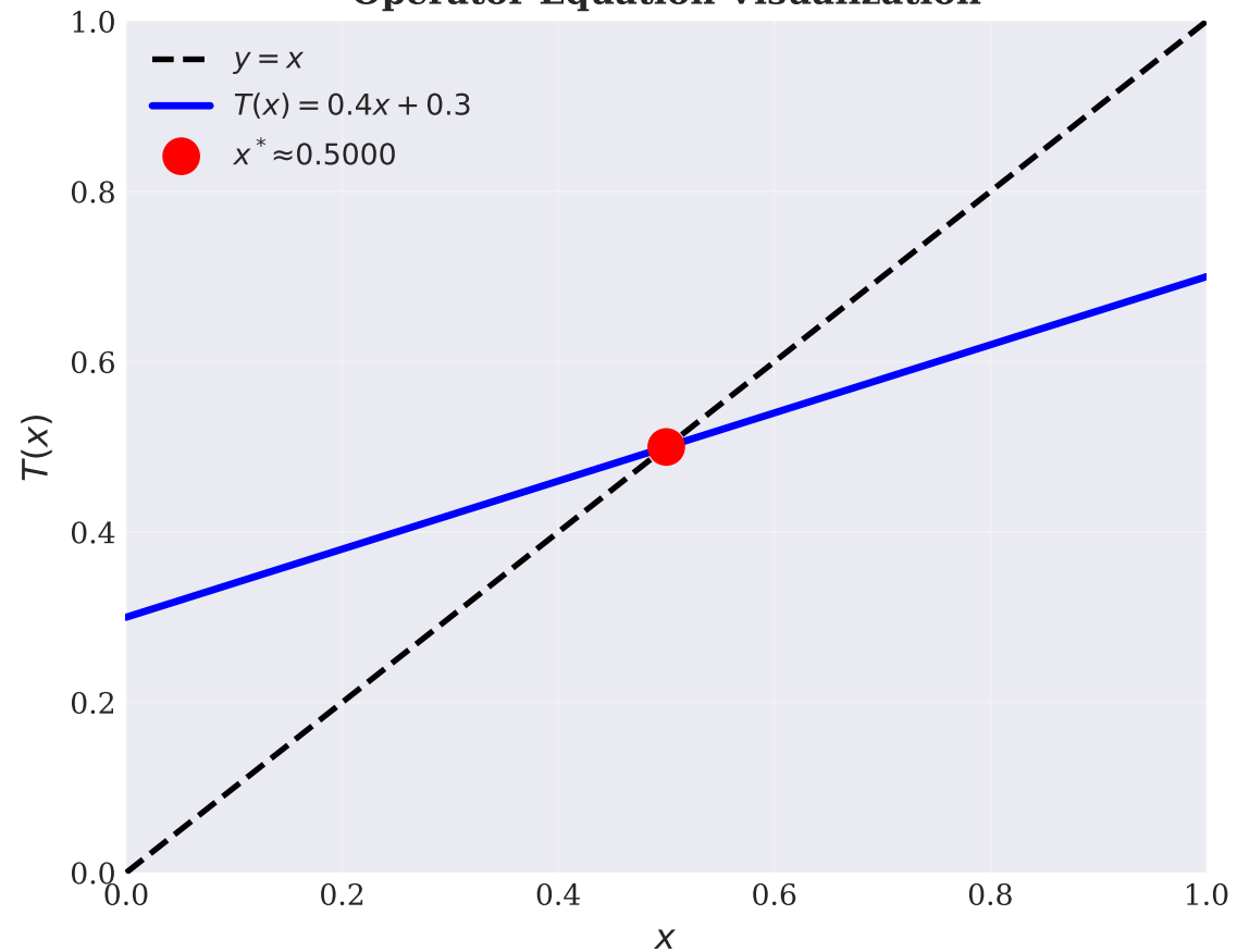
Operator Equation Visualization
