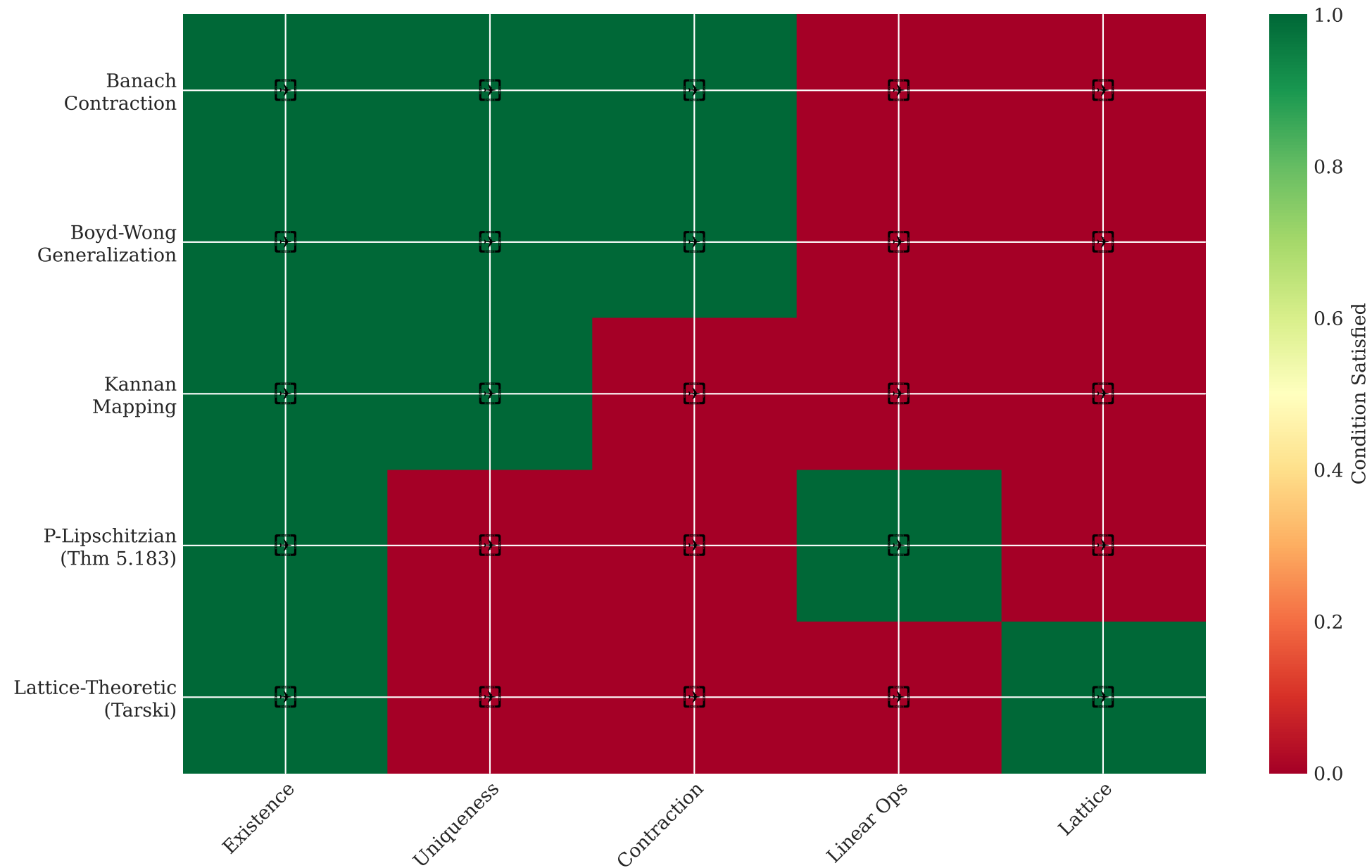
Comparison of Fixed Point Theorem Conditions
