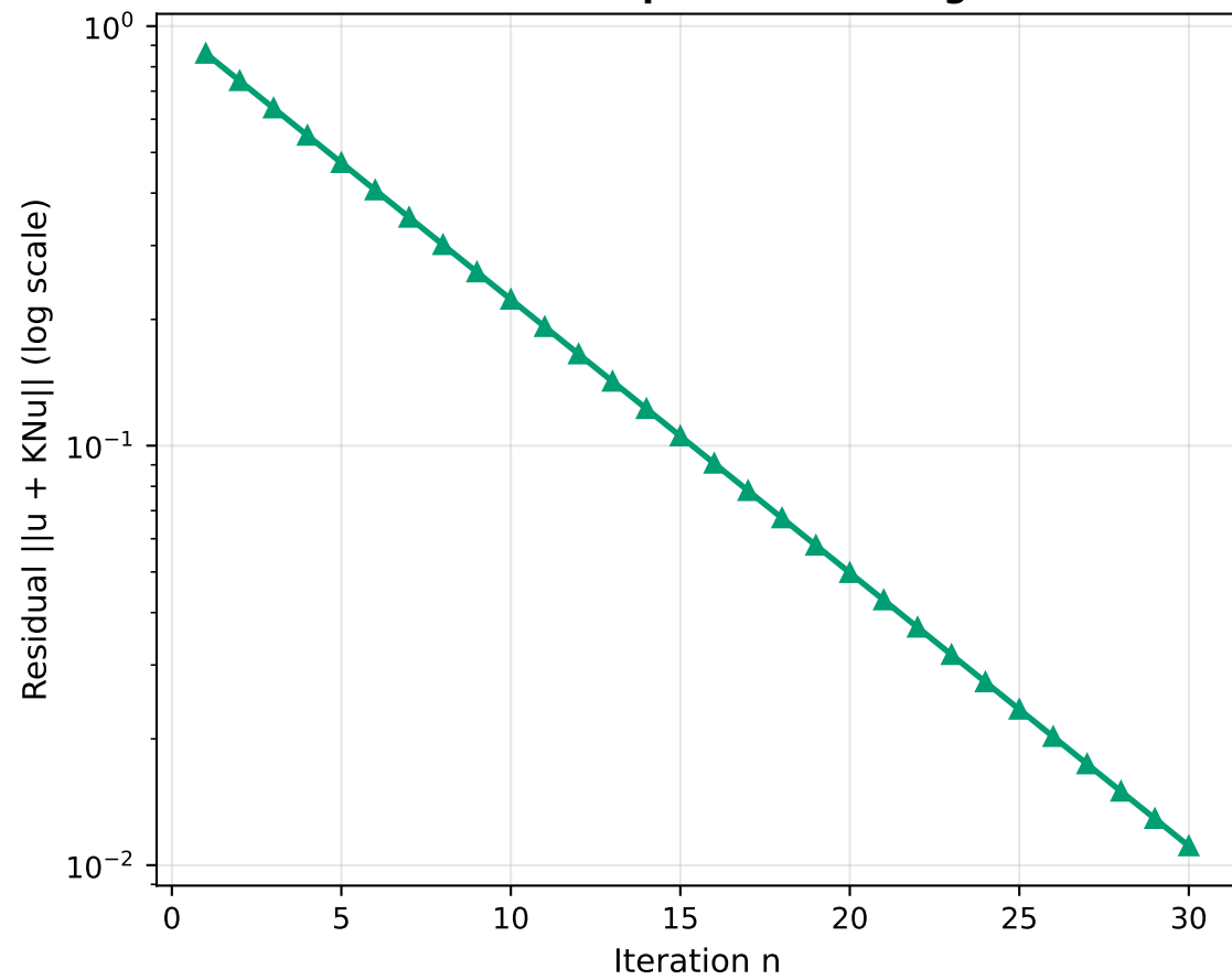
Hammerstein Operator Convergence
