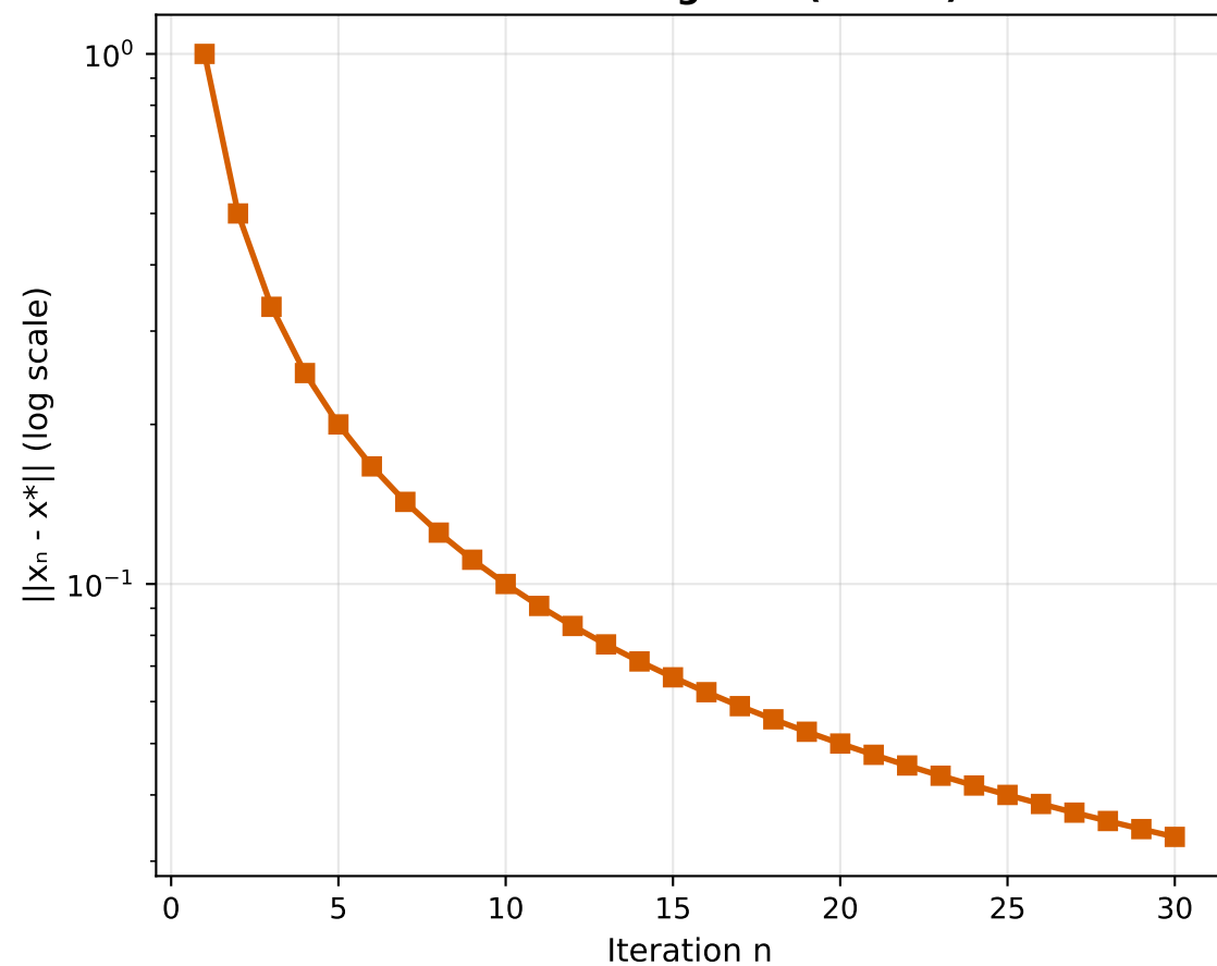
Contraction Mapping: \rho^n Decay
