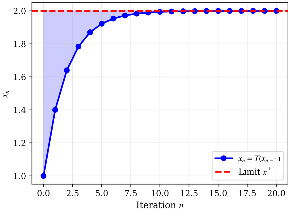
Convergence to Fixed Point
