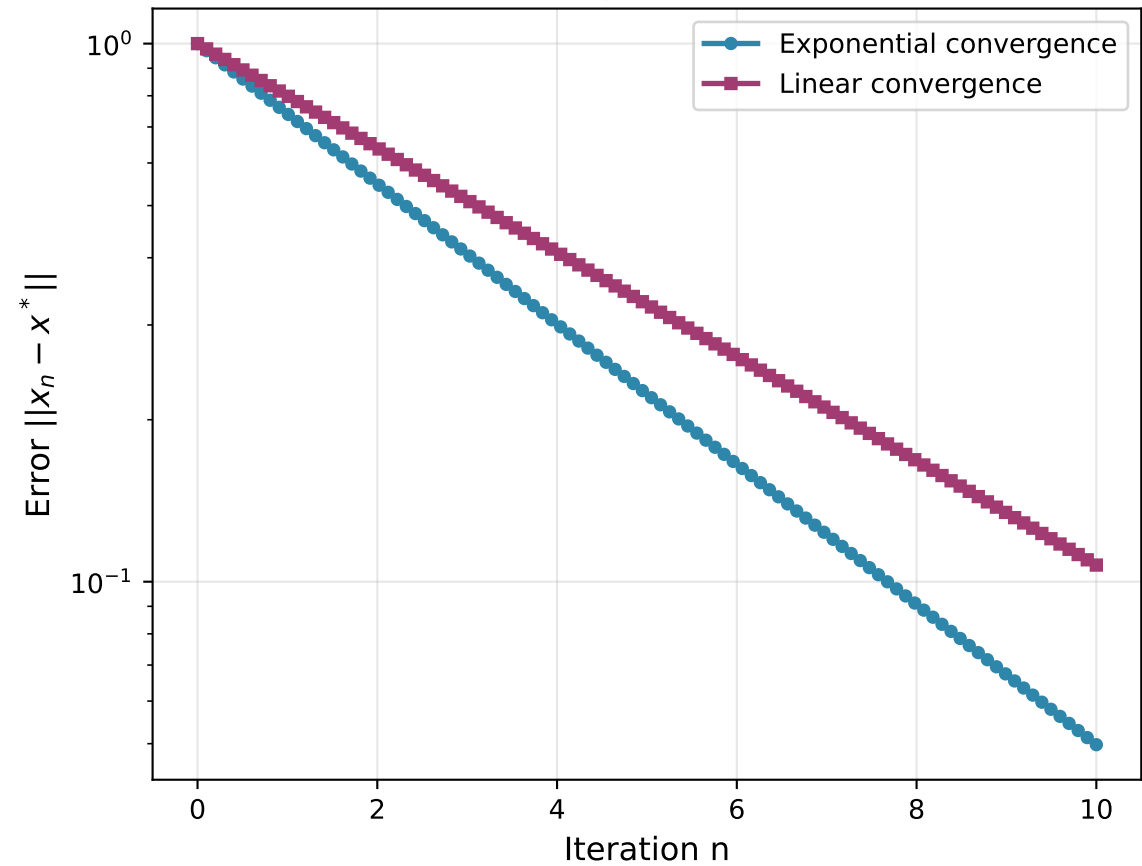
Convergence Rates
