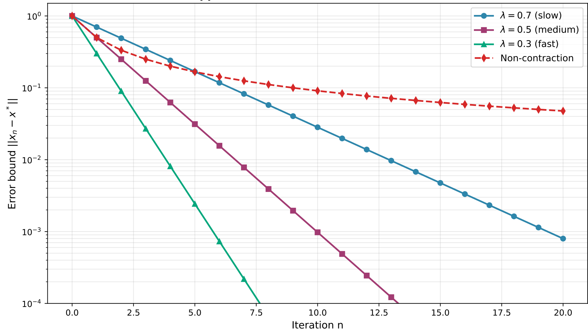
Approximation Error vs. Contraction Rate
