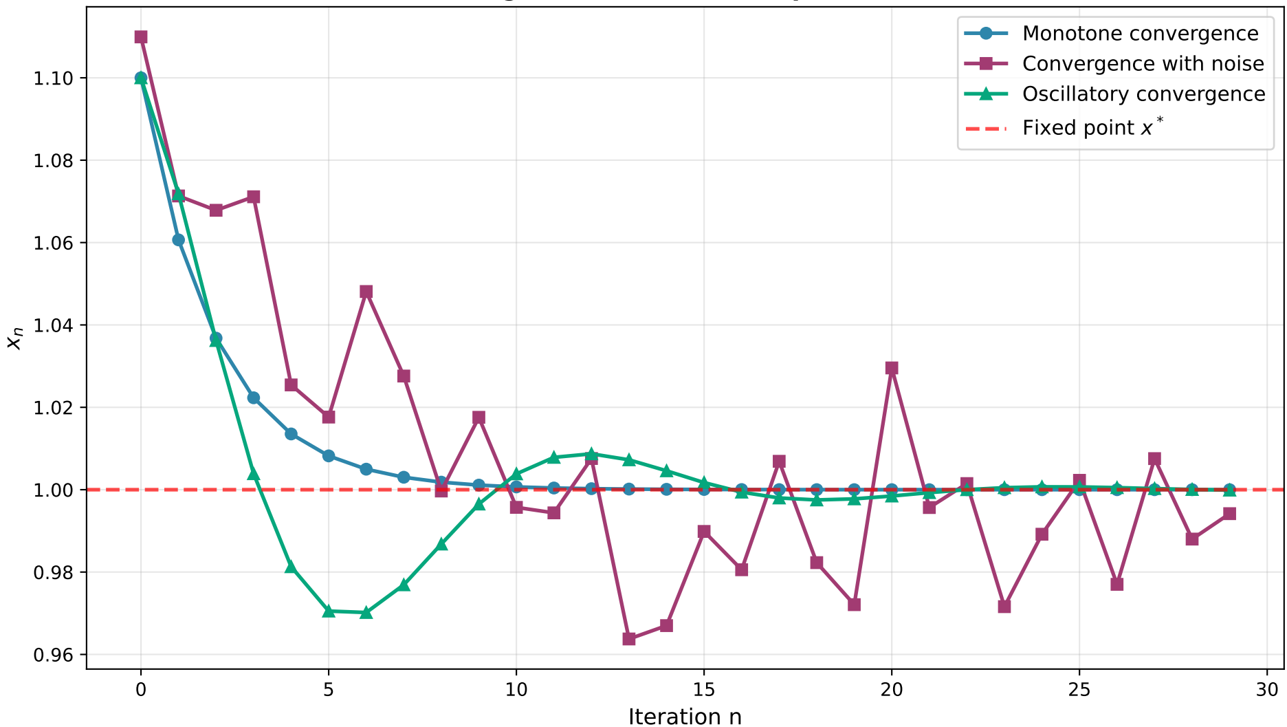
Convergence of Iterative Sequences \{x_n\}
