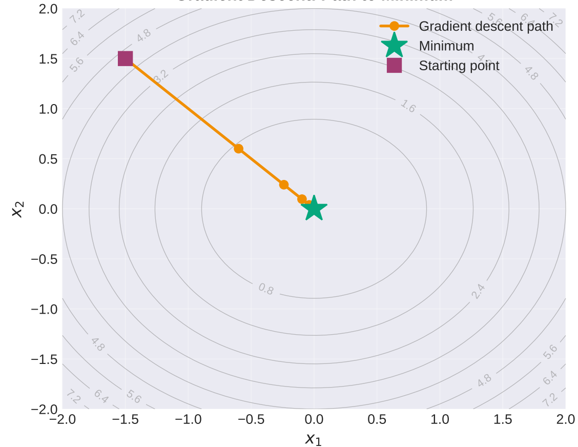
Gradient Descent: Path to Minimum
