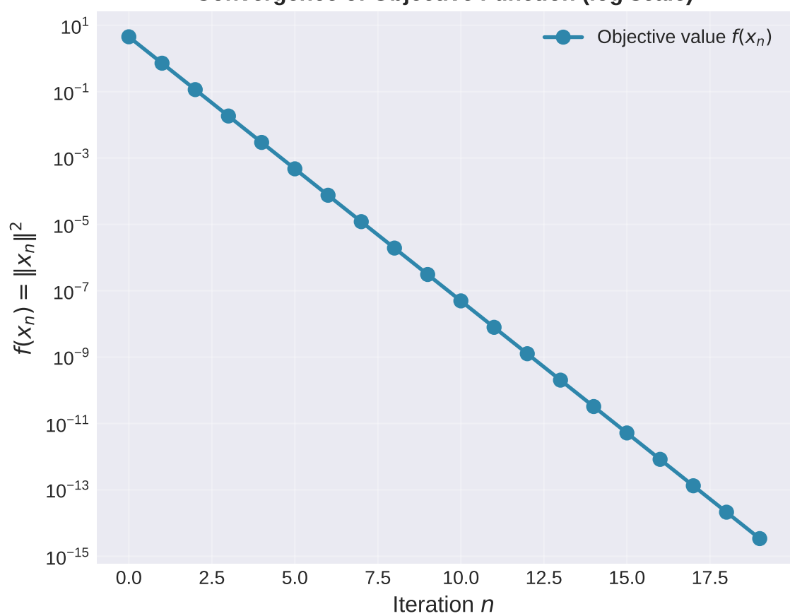
Convergence of Objective Function (log scale)
