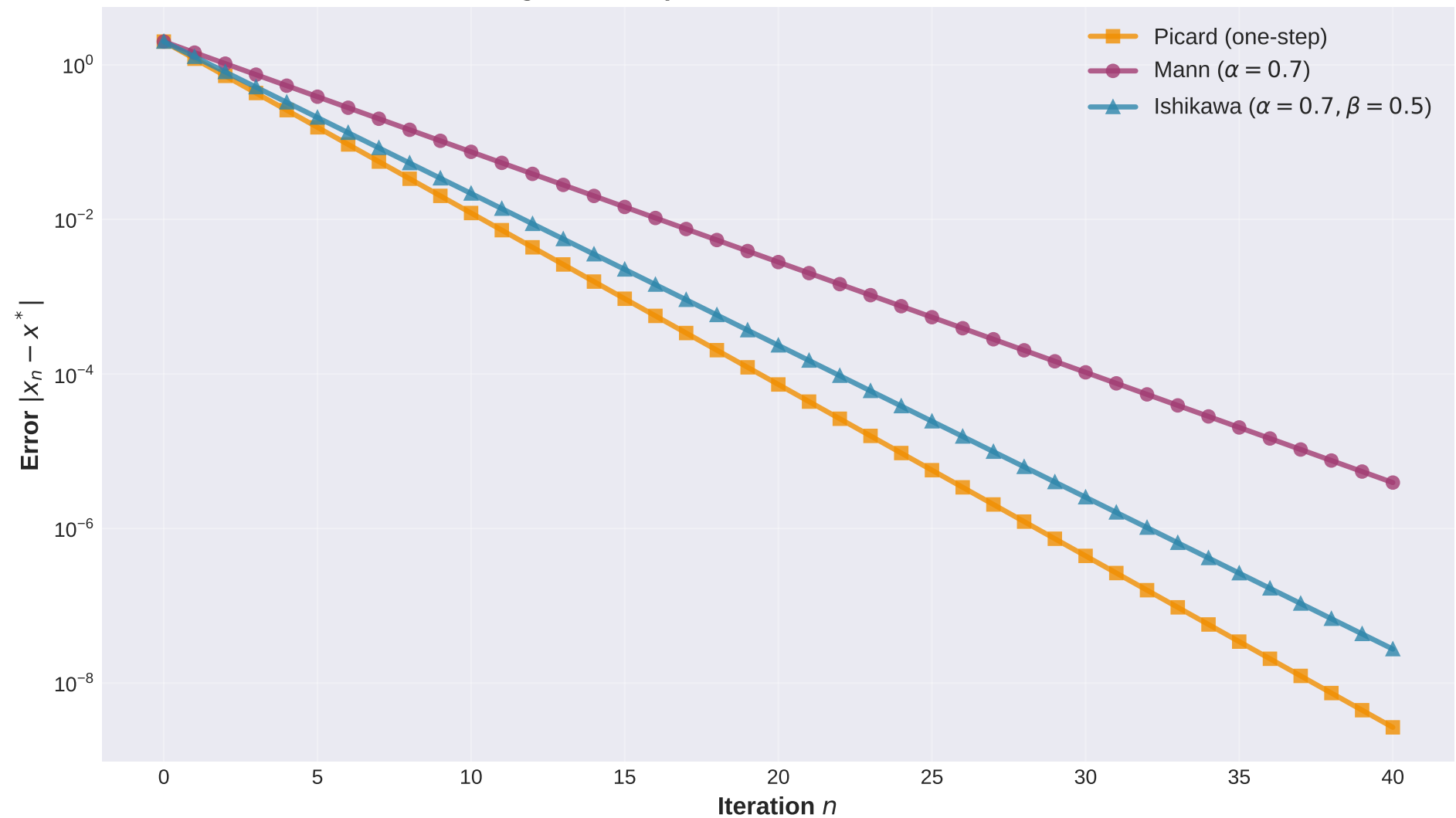
Convergence Comparison: Picard vs Mann vs Ishikawa
