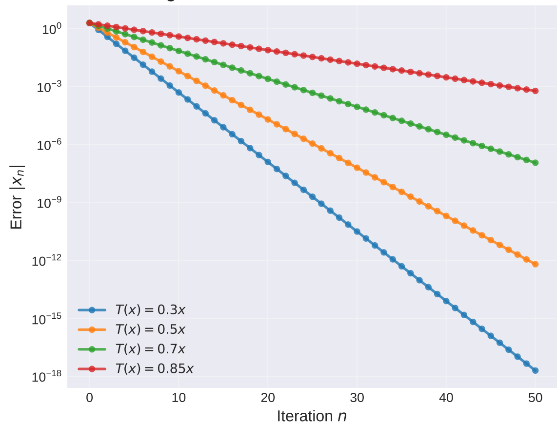
Convergence for Different Contraction Coefficients
