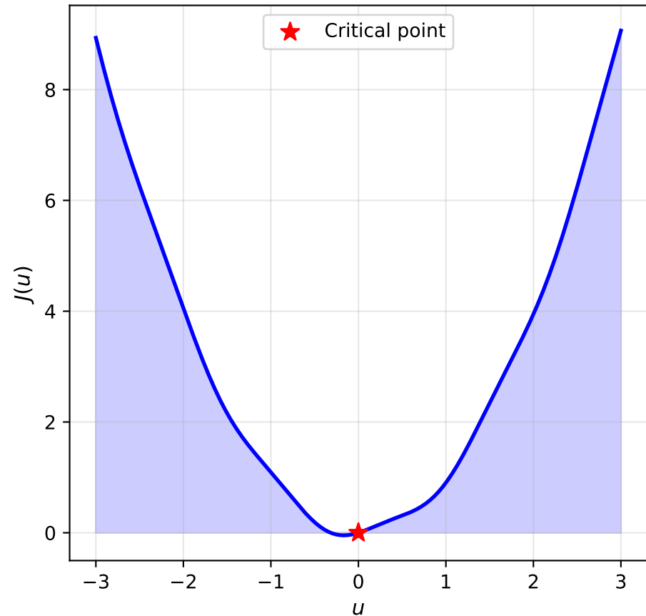
Satisfies Palais-Smale (PS)
