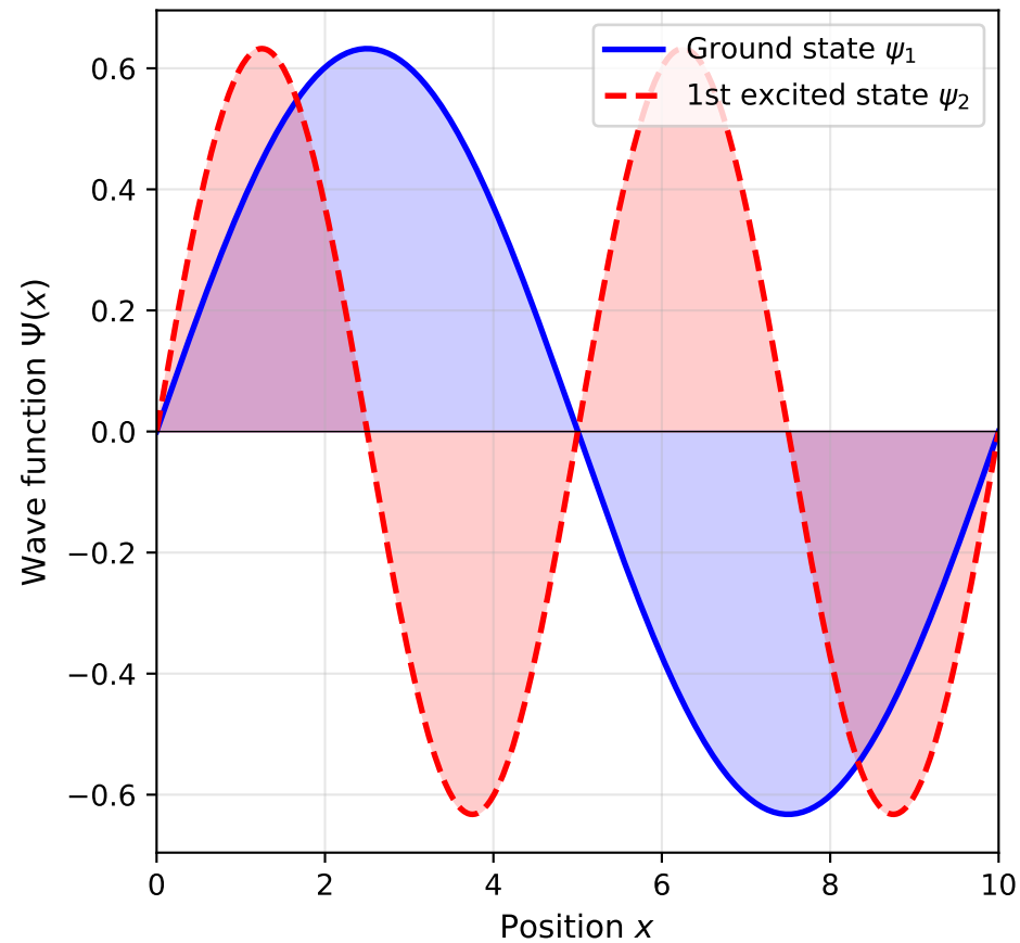
Wave Functions: Particle in a Box
