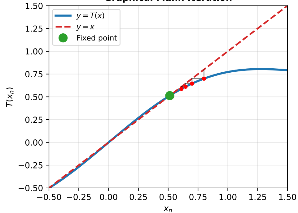
Graphical Mann Iteration
