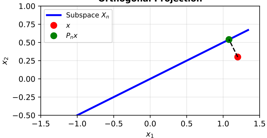
Orthogonal Projection
