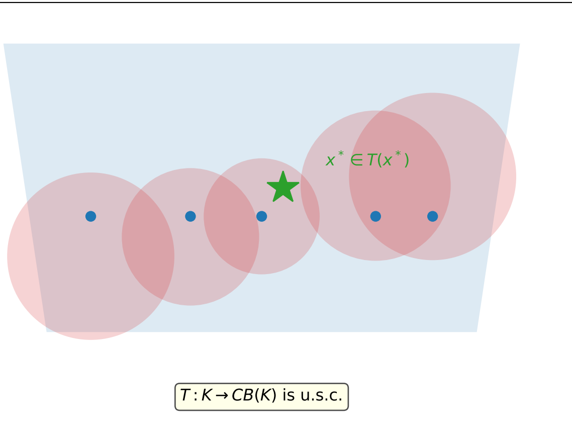
Fixed Point in Compact Convex Set
