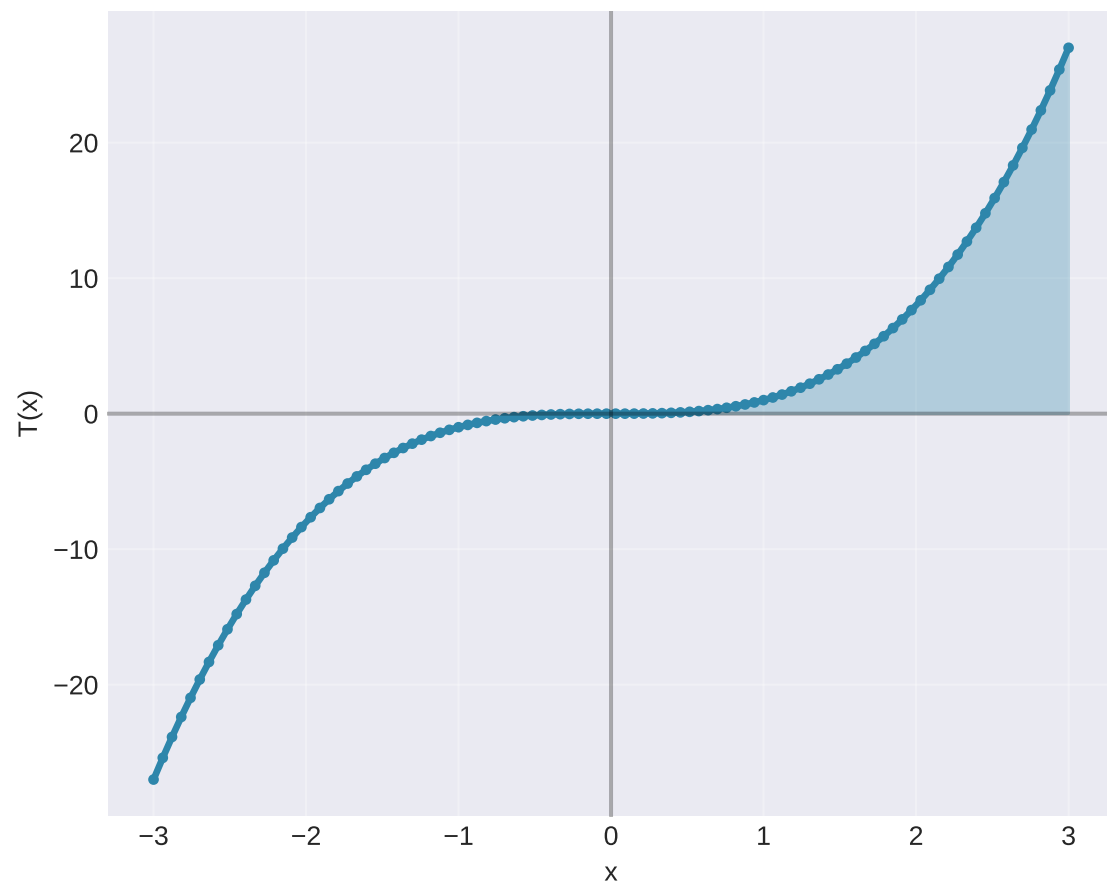
Monotone: \langle T(x) - T(y), x - y \rangle \geq 0
