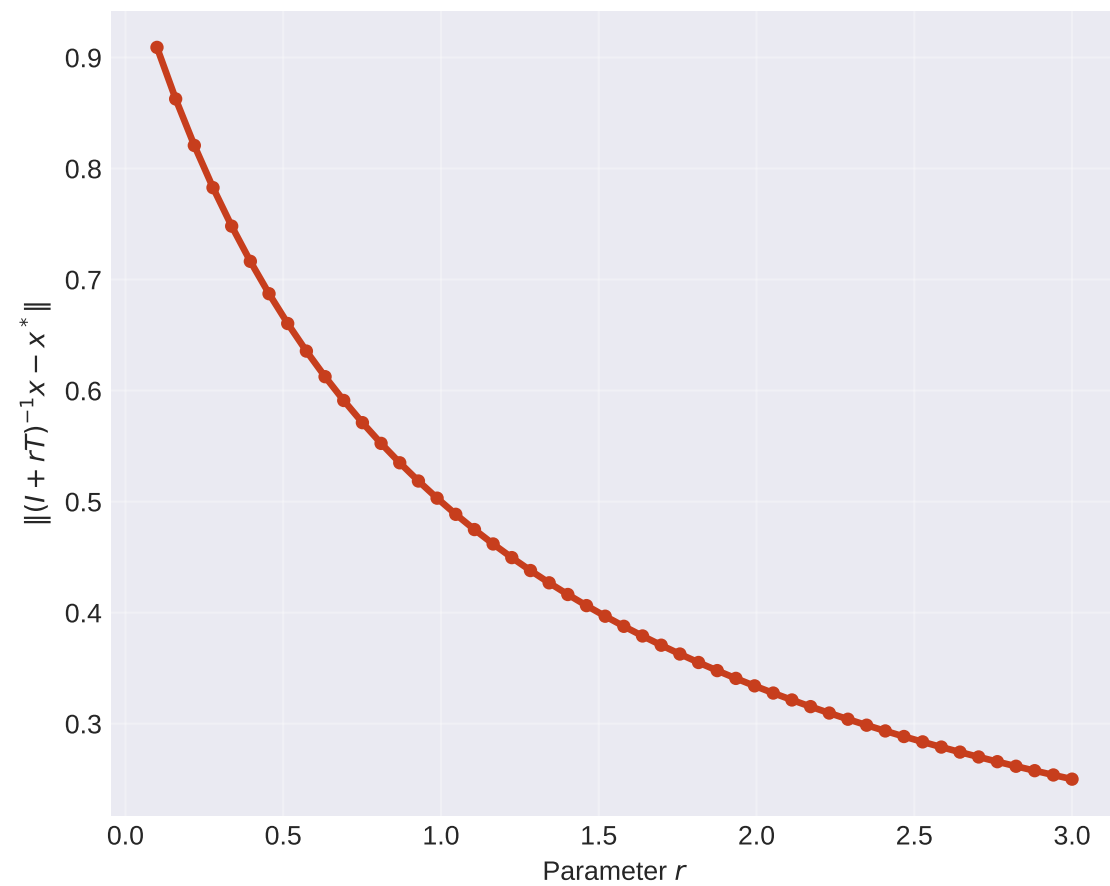
Resolvent (I + rT)^{-1} Error vs r
