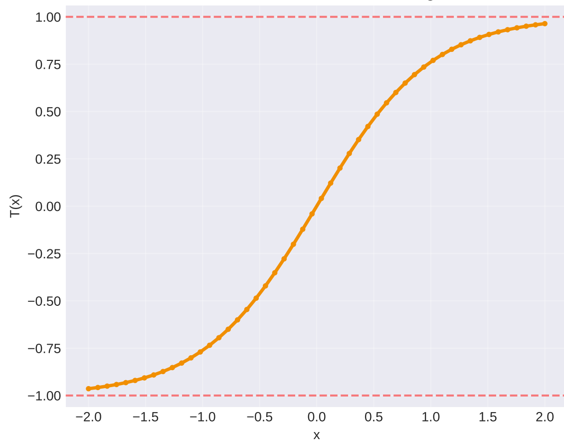
Maximal Monotone: Bounded Range
