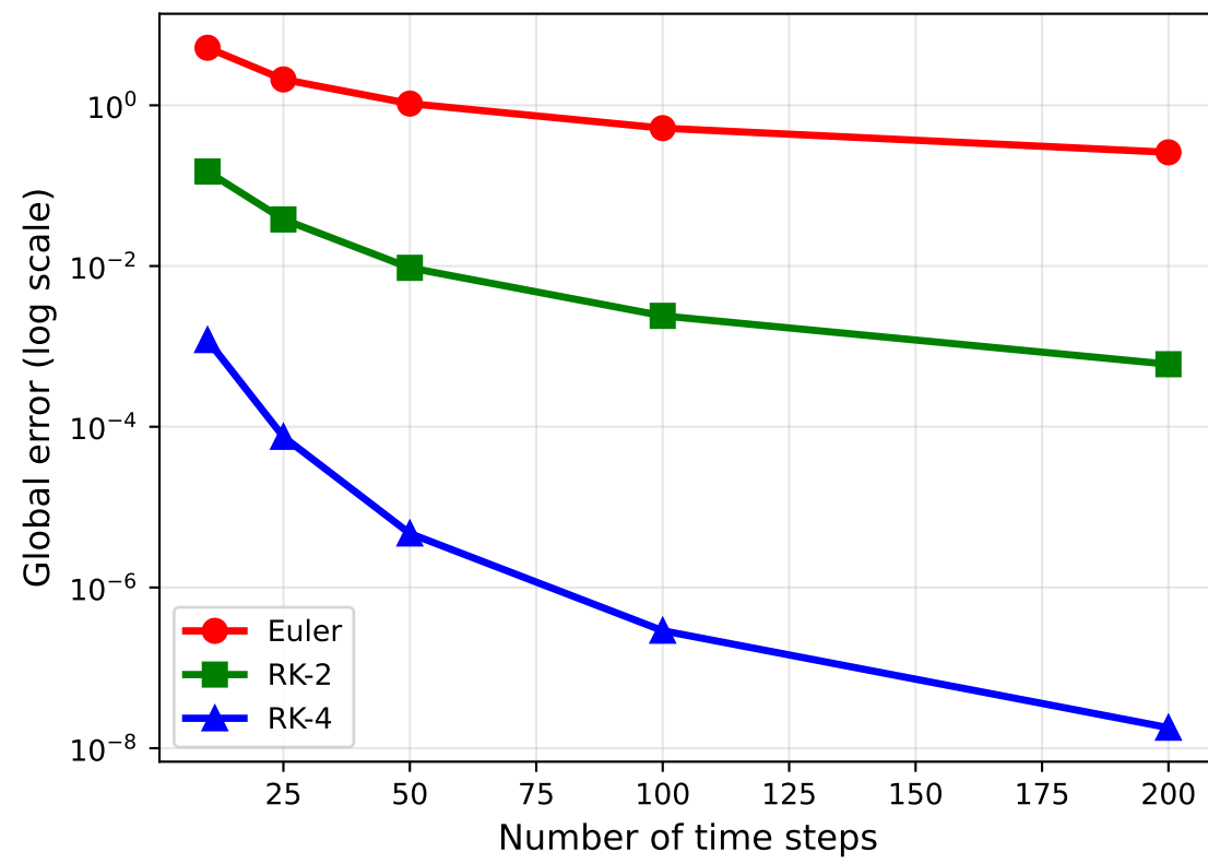
Global Error Accumulation
