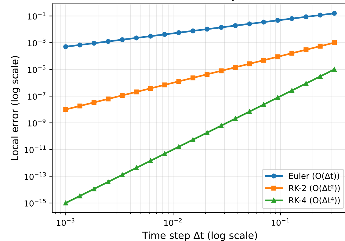
Error vs Time Step Size
