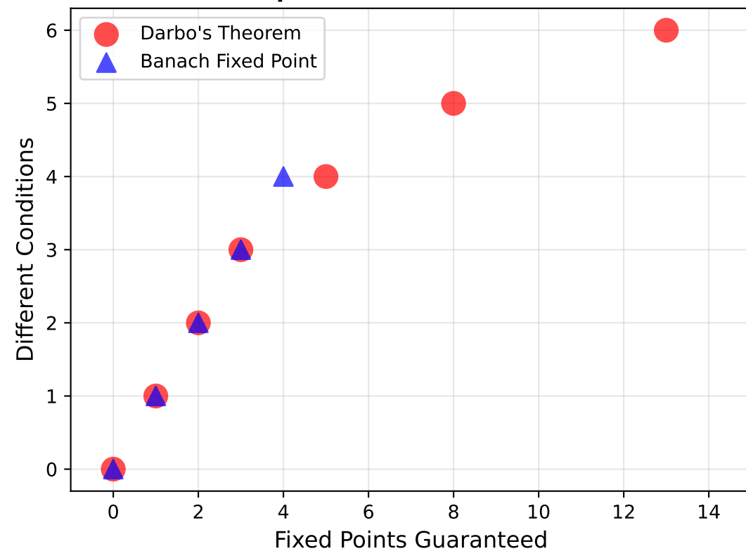
Comparison: Darbo vs Banach
