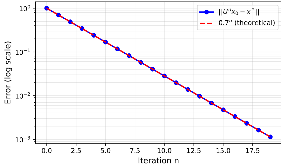
Convergence Rate: Contraction Mapping
