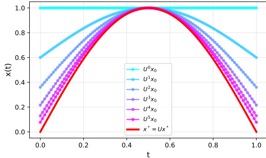
Fixed Point Iteration: U^n x_0 \rightarrow x^*
