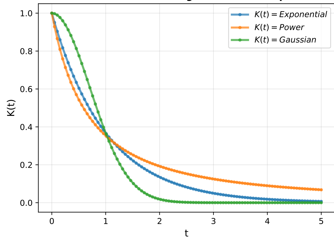
Kernel Functions for Integrodifferential Equations
