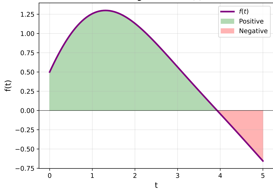
Forcing Function: f(t)
