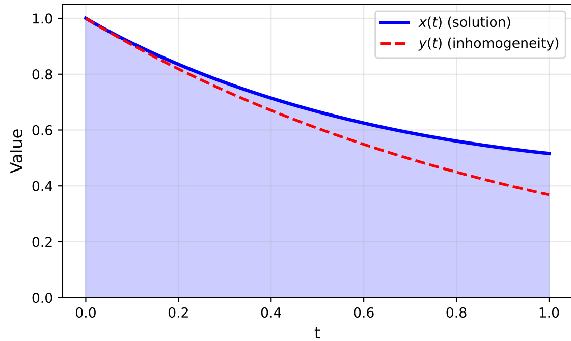
Urysohn Integral Equation Solution
