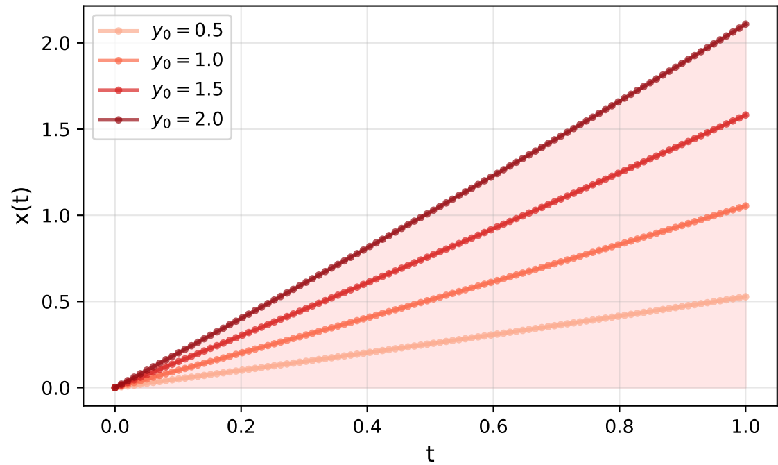
Cone Positivity: x \geq 0 (when y \geq 0 , K \geq 0 )
