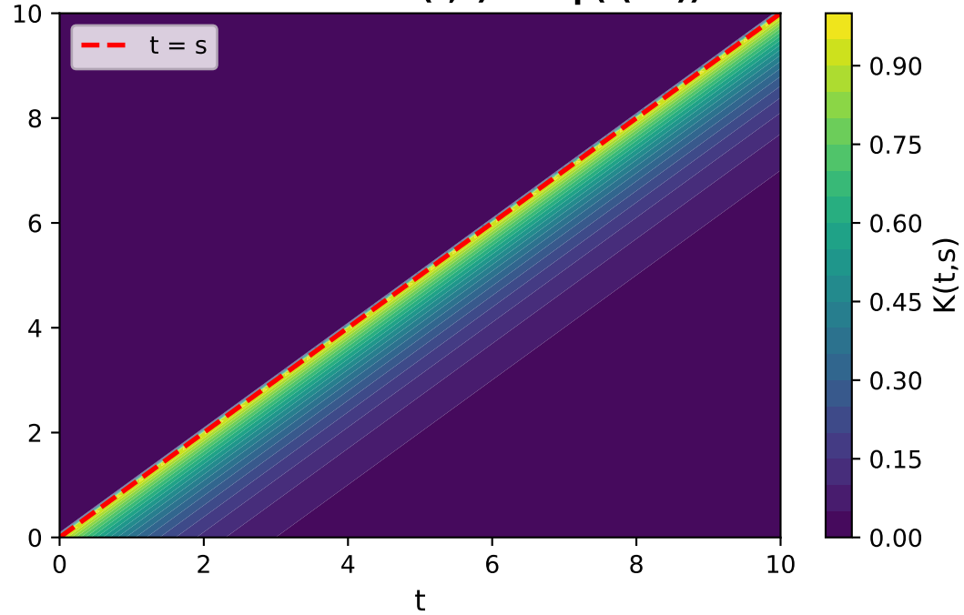
Volterra Kernel K(t,s) = \exp(-(t-s))
