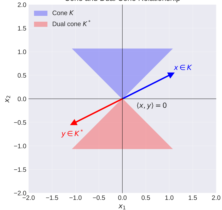
Cone and Dual Cone Relationship
