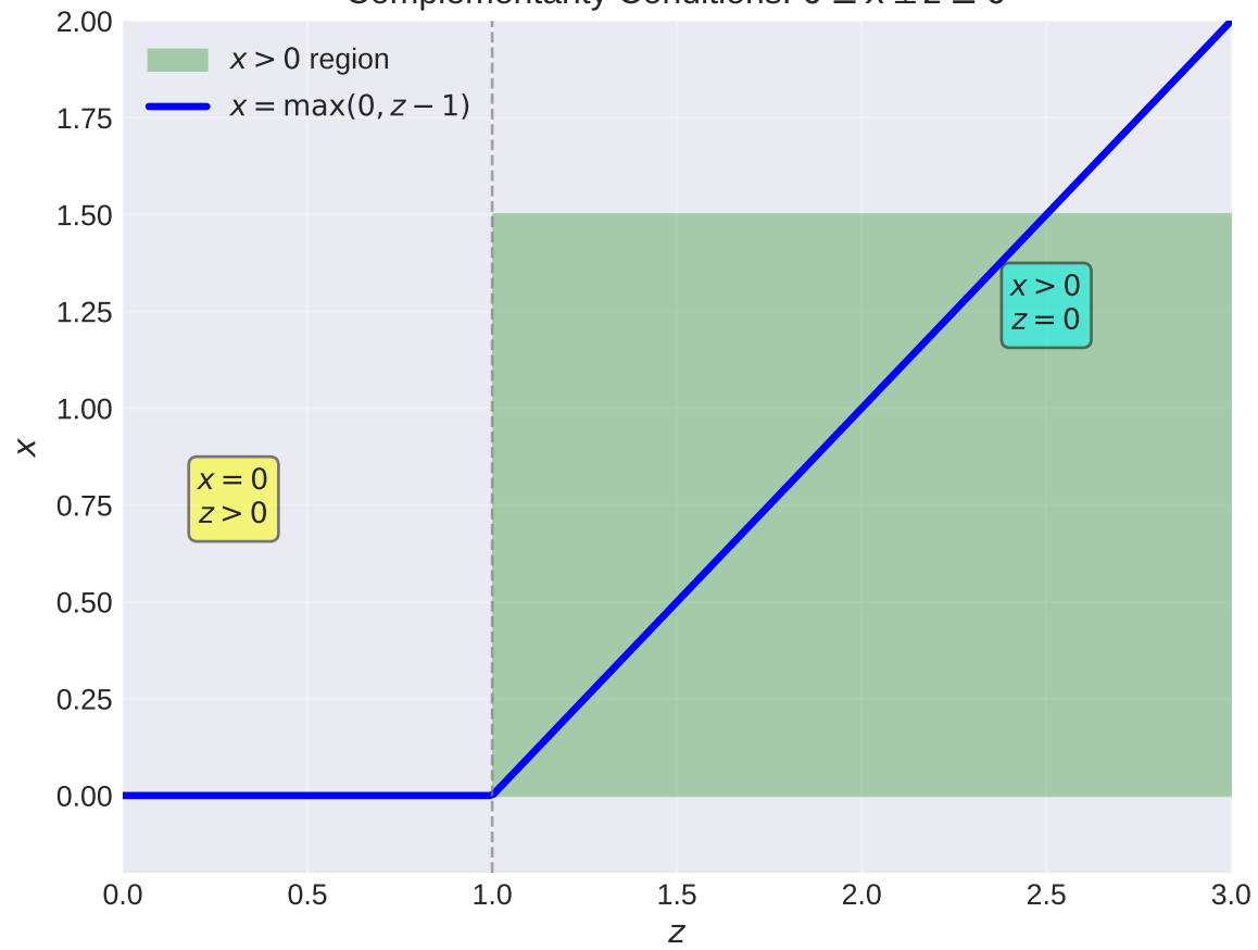
Complementarity Conditions: 0 \leq x \perp z \geq 0
