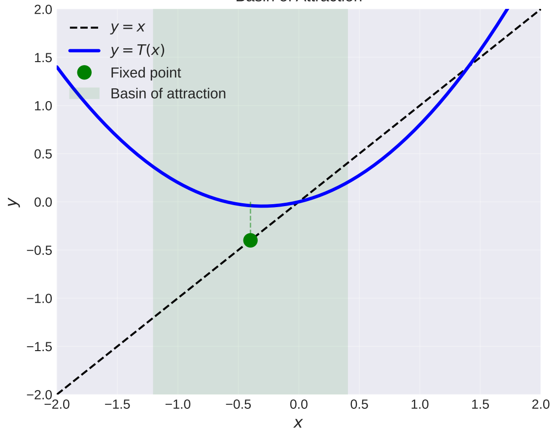
Basin of Attraction
