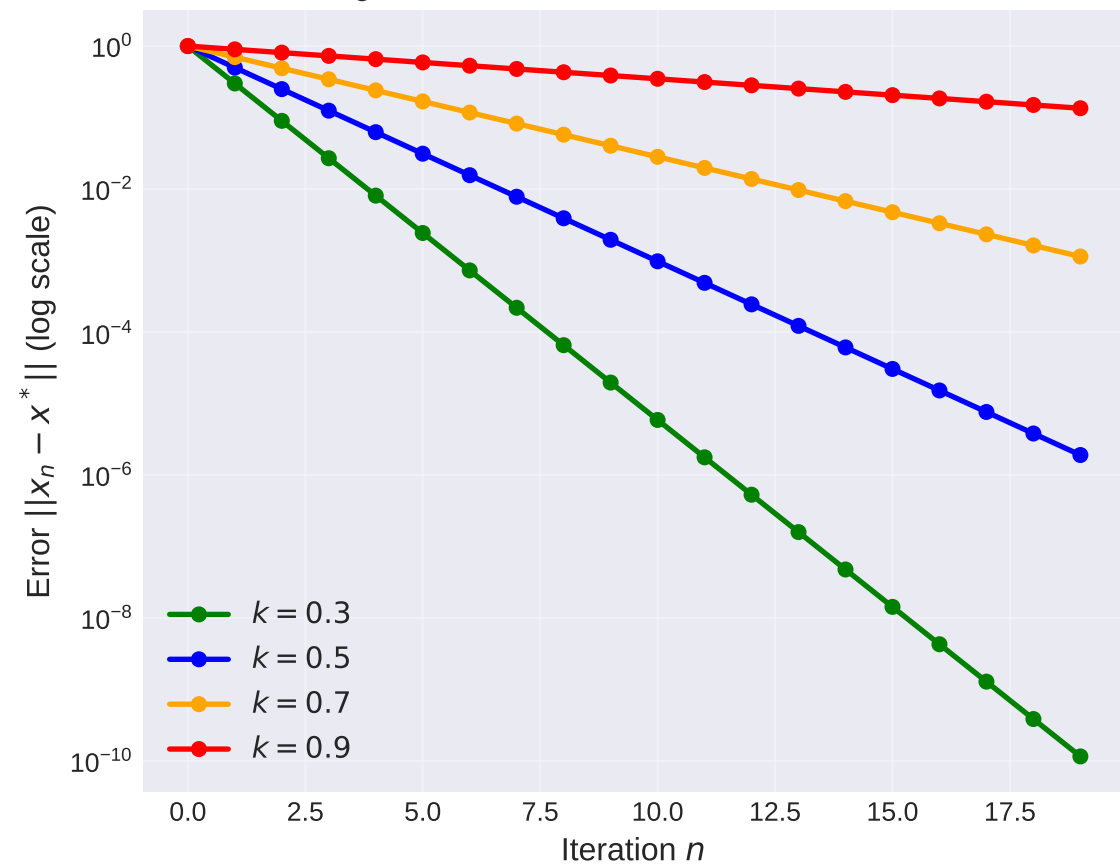
Convergence Rate for Different Contraction Constants
