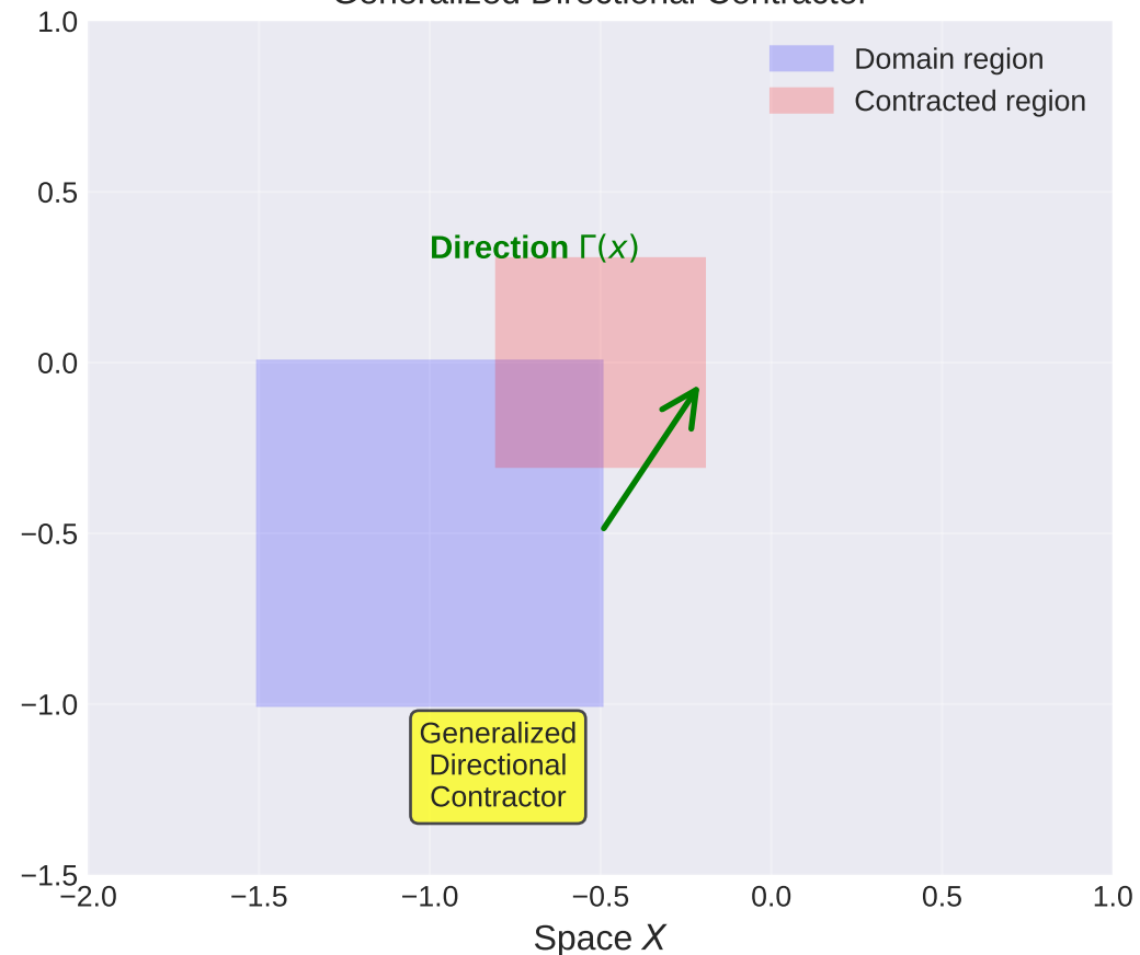
Generalized Directional Contractor
