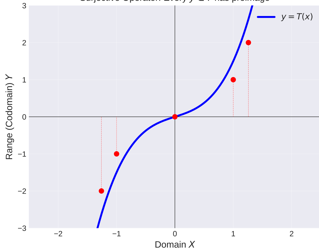
Surjective Operator: Every y \in Y has preimage
