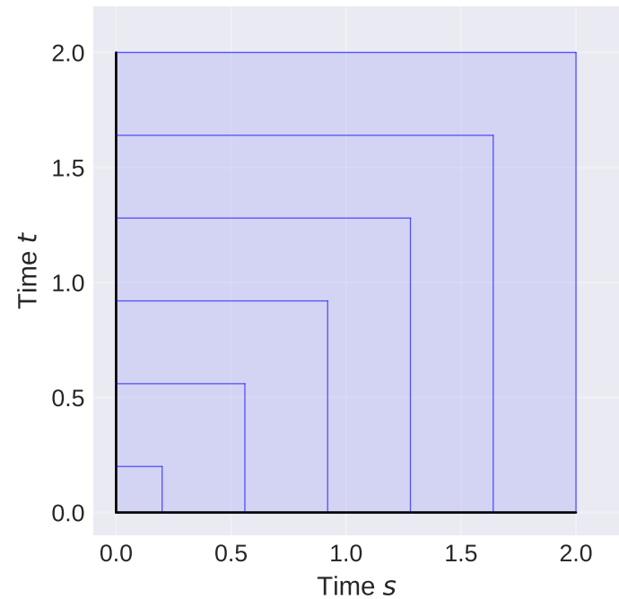
Volterra Integral Domain: 0 \leq s \leq t
