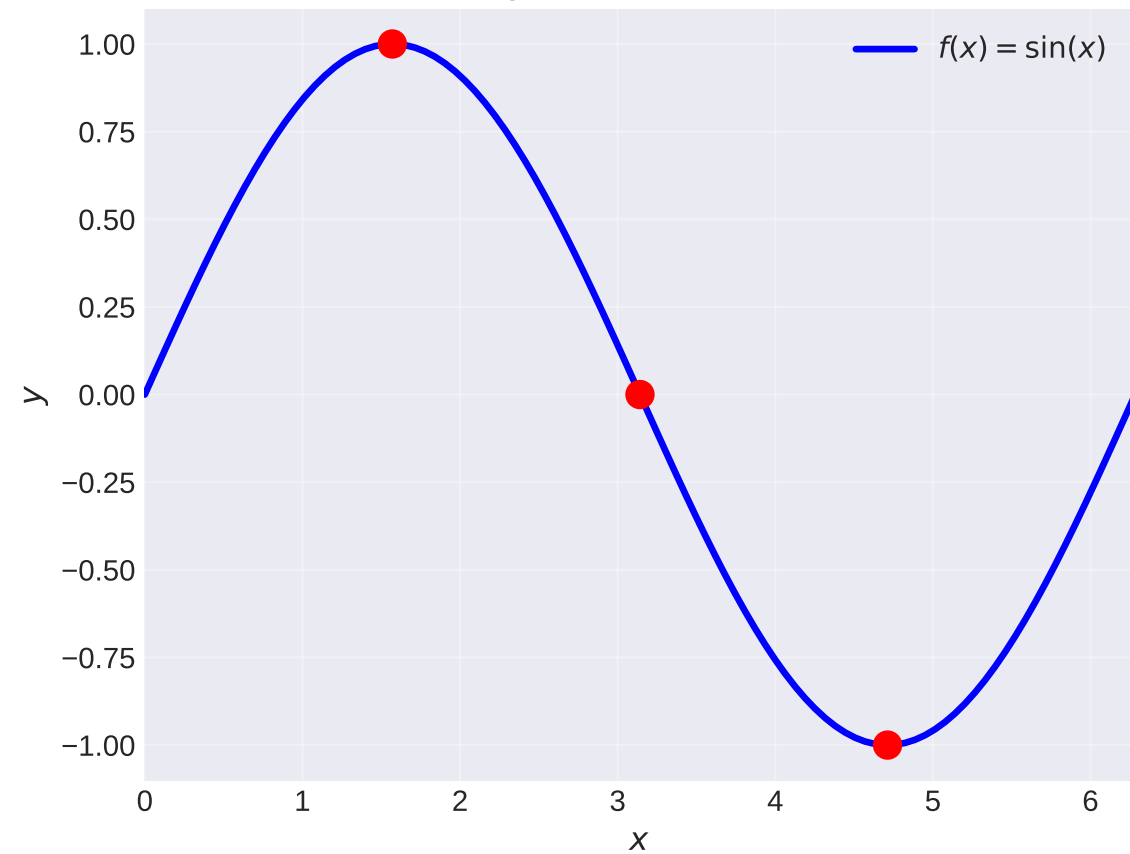
Single-Valued Function
