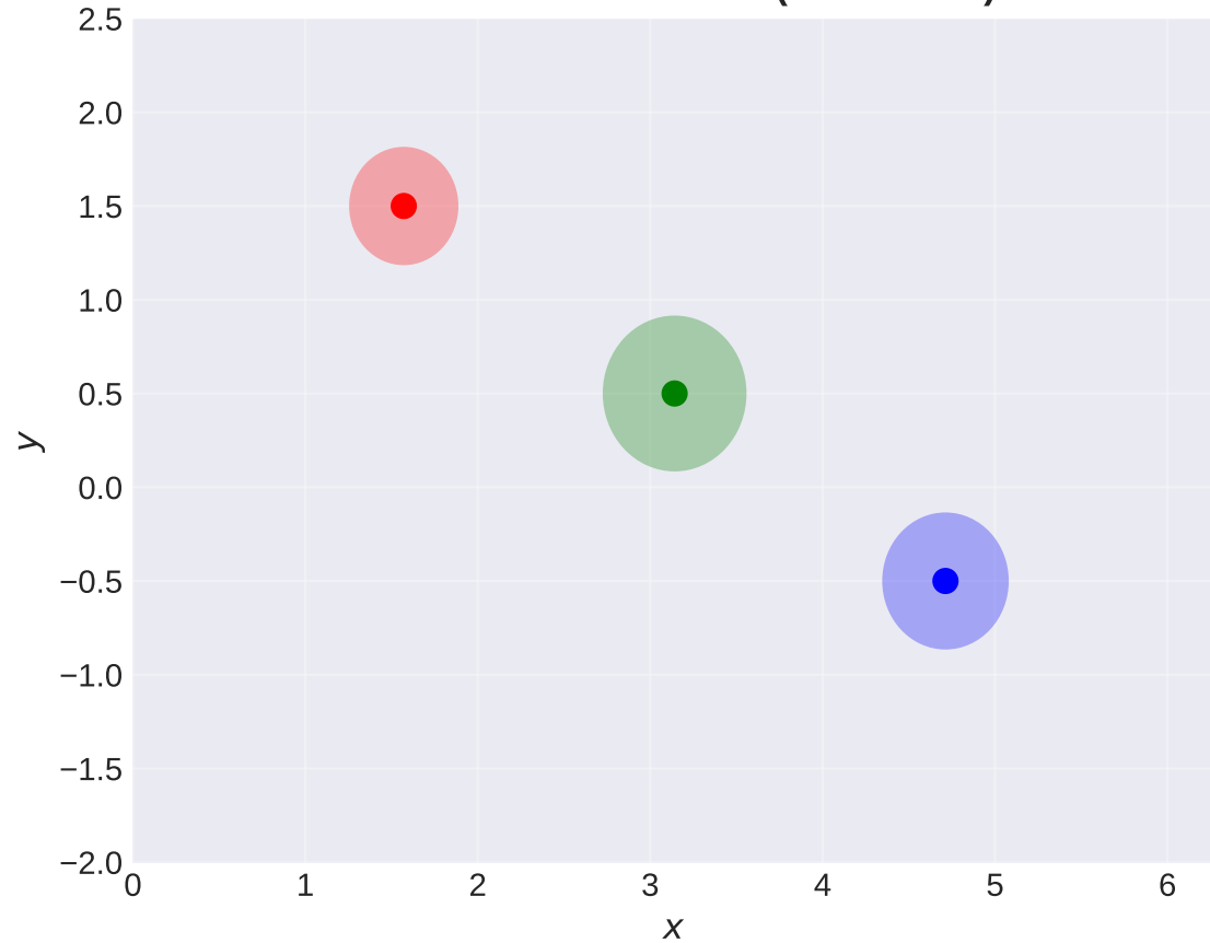
Multifunction F : X \rightarrow 2^Y (Set-Valued)
