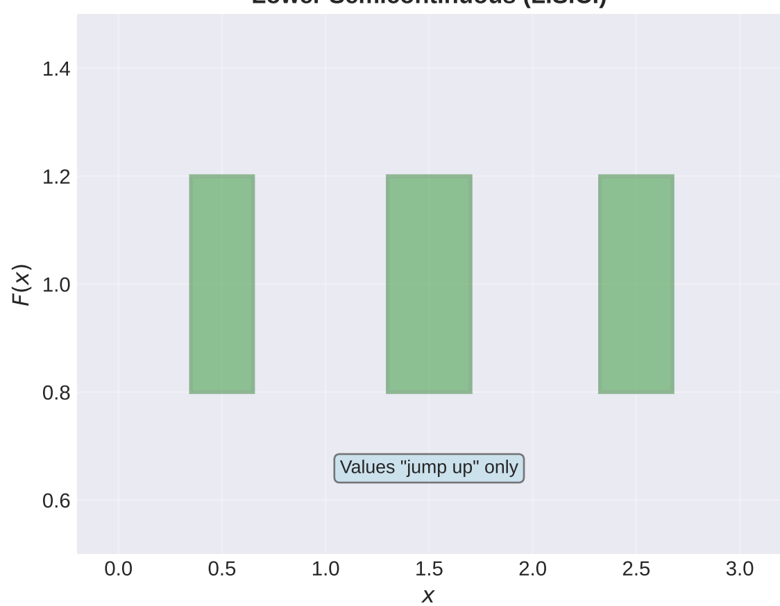
Lower Semicontinuous (L.S.C.)
