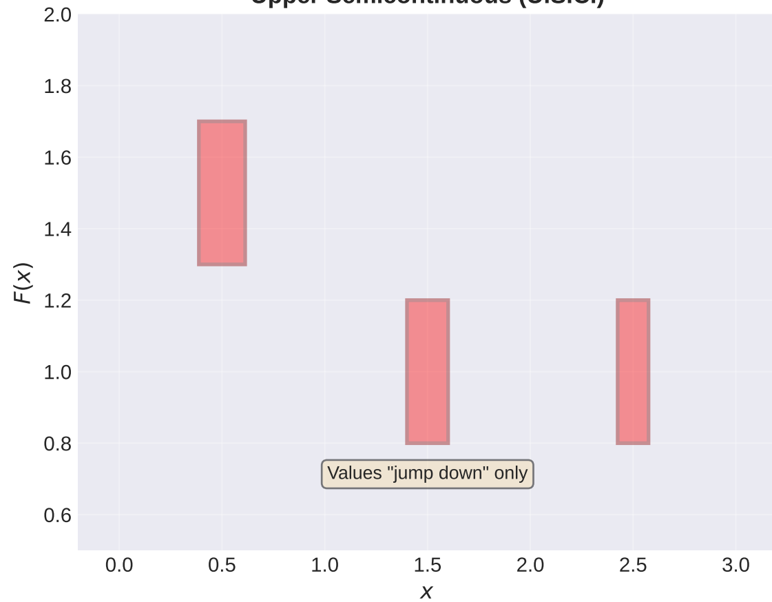
Upper Semicontinuous (U.S.C.)
