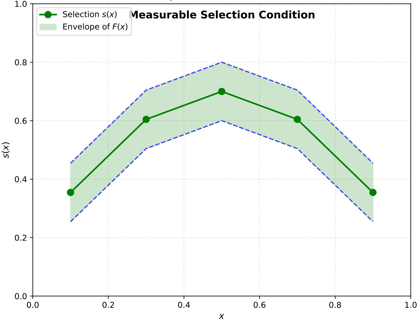
Graph of Measurable Selection
