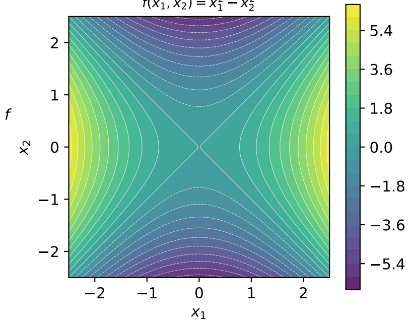
Contour Plot: f(x_1, x_2) = x_1^2 - x_2^2
