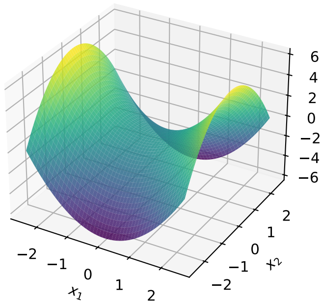
3D Surface: f(x_1, x_2) = x_1^2 - x_2^2
