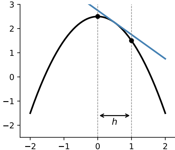
Forward difference
