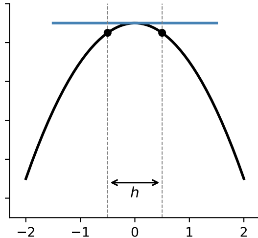
Central difference
