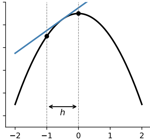
Backward difference
