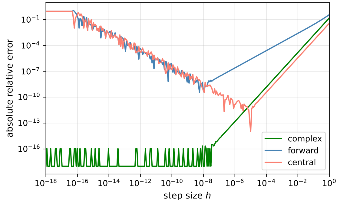
Derivative error for \sin(x) at x = 0.5
