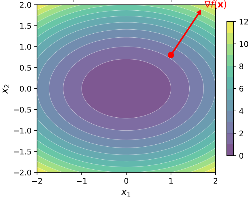
Gradient points in direction of steepest ascent
