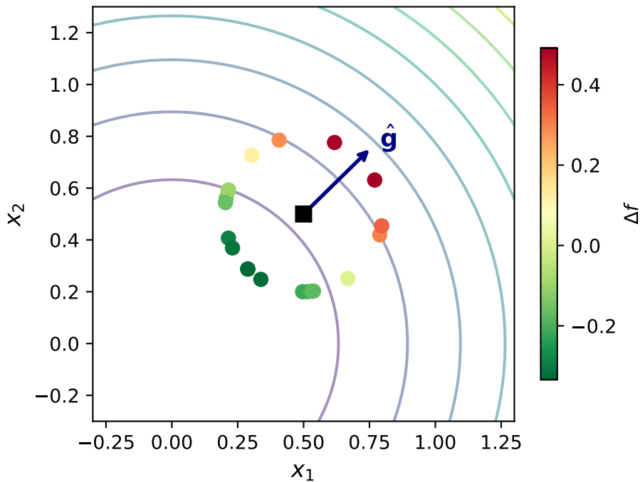
Regression gradient (m=20 perturbations)
