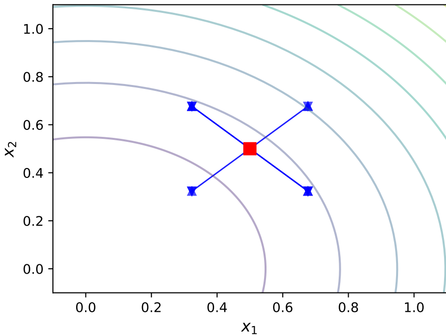
SPSA: symmetric perturbation pairs
