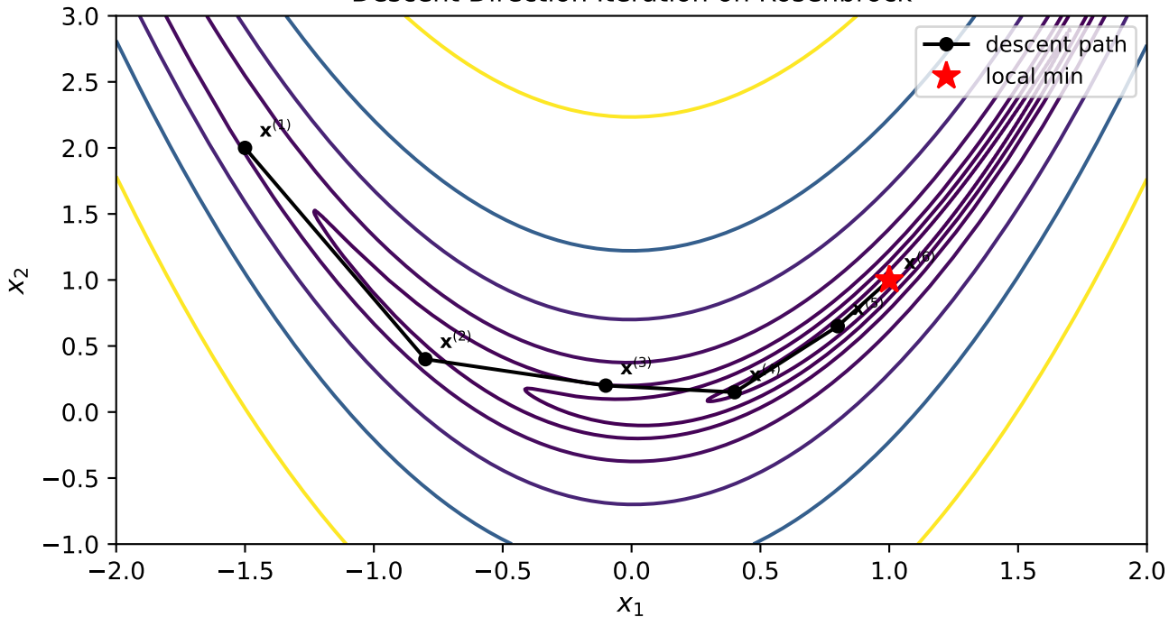
Descent Direction Iteration on Rosenbrock
