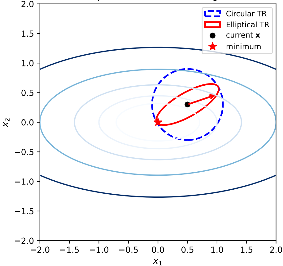
Elliptical vs Circular Trust Region
