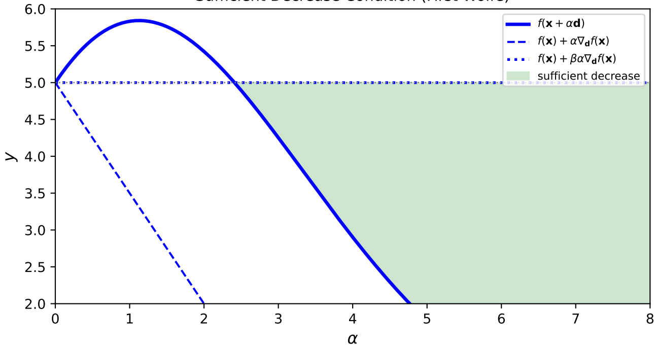
Sufficient Decrease Condition (First Wolfe)
